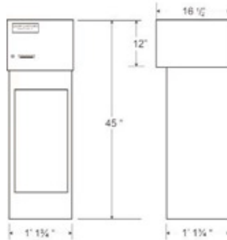
Housing Dimension
